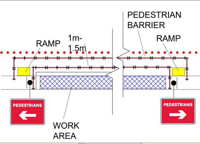
PEDESTRIAN WALKWAY DETAIL
